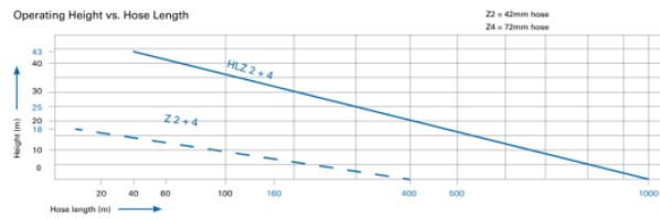
Operating Height vs. Hose Length
