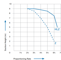
Suction Height vs. Proportioning Rate
